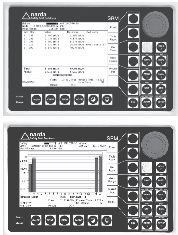
The UMTS P-CPICH Demodulation Option allows the SRM to decode all the pilot channels (P-CPICH) contained in a 5 MHz bandwidth UMTS frequency block and can thus correlate the measured field strengths to the respective pilot channels.
