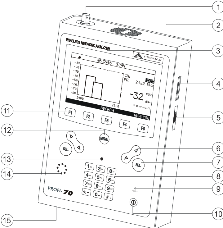
Figure 2.- Front panel.
