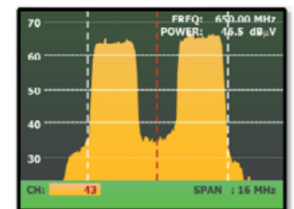
Spectrum hole unveiling the presence of intermodulation products within the channel
