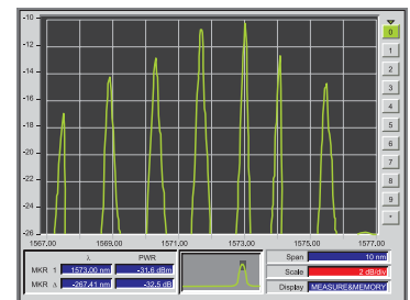
Spectrum of a measured WDM system using a PROLITE-60 from PROMAX
