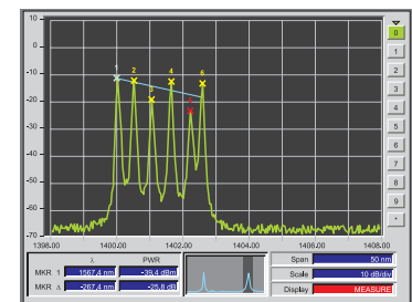
Automatic measurement of a WDM system using a PROLITE-60
